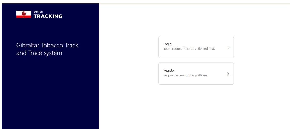
Figure 7 – Onboarding Wizard
